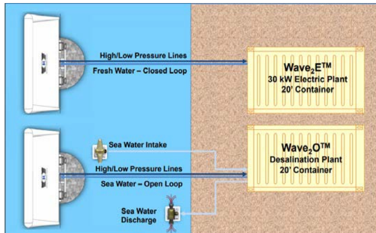
Figure 7.3. Configuration of Resolute Marine's Wave20 desalination system. Image courtesy of Resolute Marine
