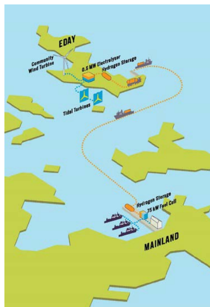
Figure 6.10. Schematic of production, transport, and storage of hydrogen gas from renewable generation for use in fuel cells at EMEC in Orkney, United Kingdom. Source: Surf 'n' Turf, European Marine Energy Center
