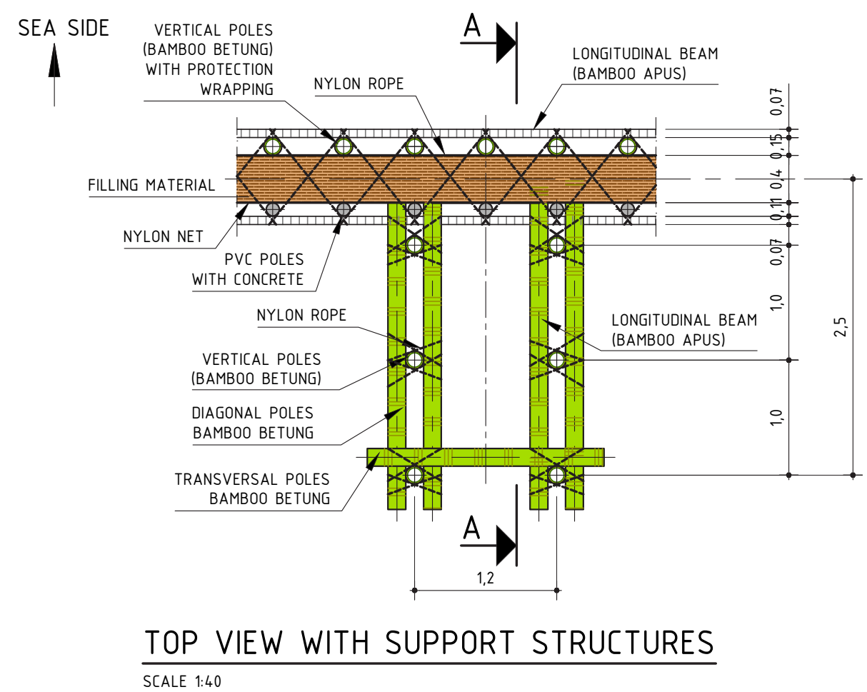
Figure 9. Configuration of the vertical poles © Witteveen+Bos
