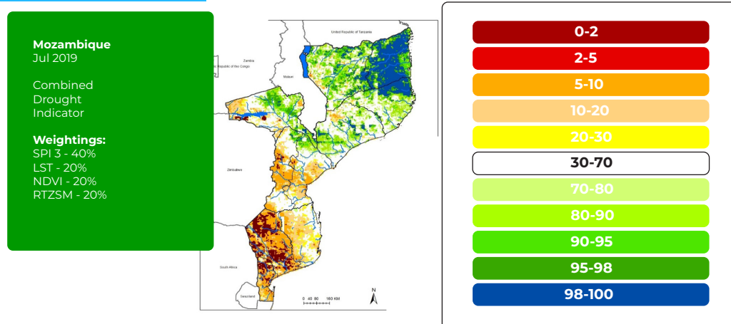
Fig 5. Combined Drought Indicator for Mozambique, July 2019
