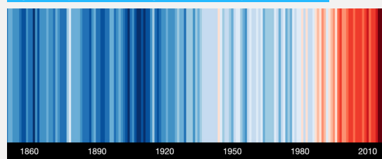
Fig 2. Temperature change in Mozambique, 1901-2019
