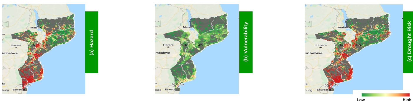
Fig 3a-c. Drought hazard, vulnerability and risk maps for Mozambique
