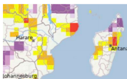
1(b) SPI-12, July 2019 to June 2020
