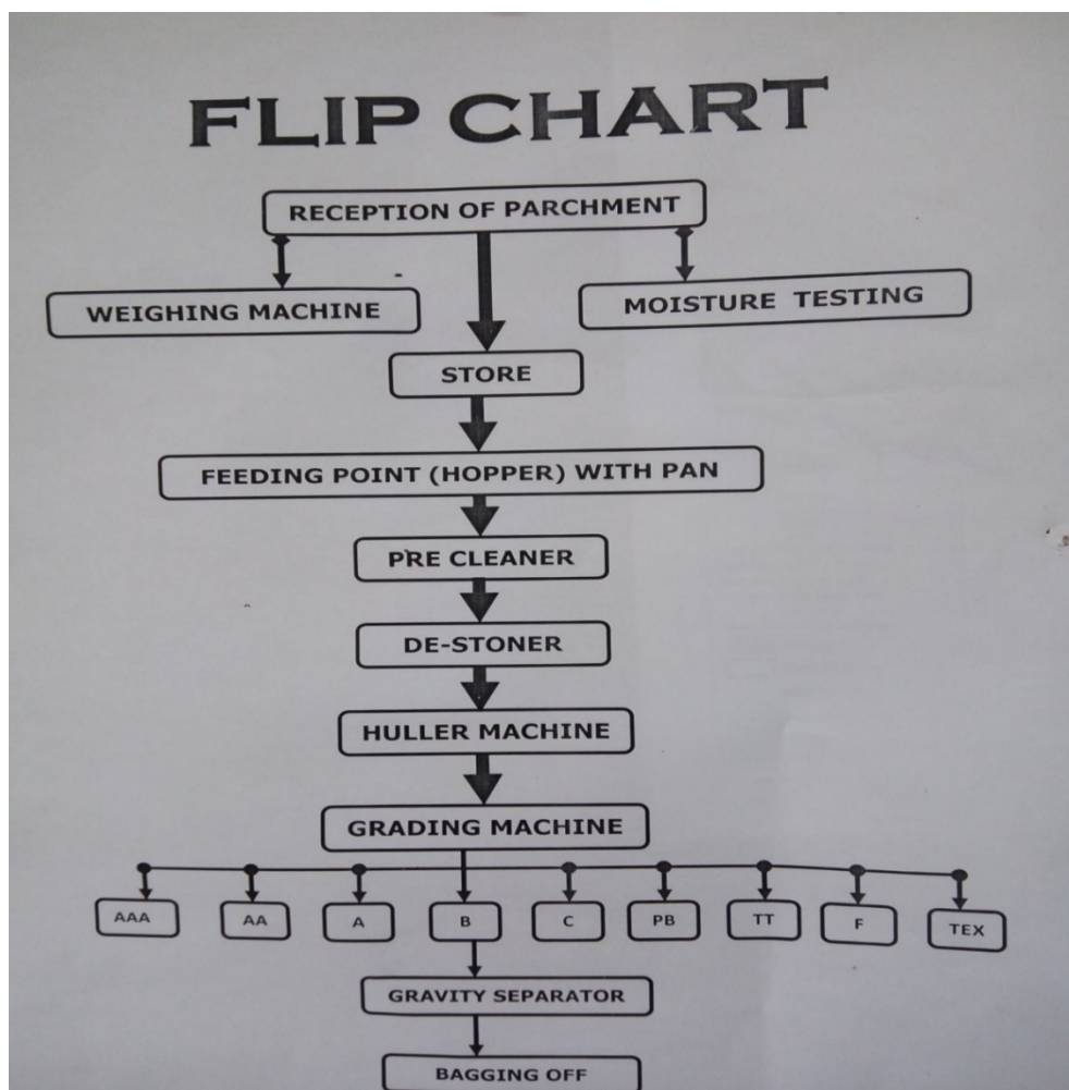
FIGURE 1.5: DRY MILLING PROCESS (SOURCE COFFEE MANAGEMENT SERVICE, 2018)
