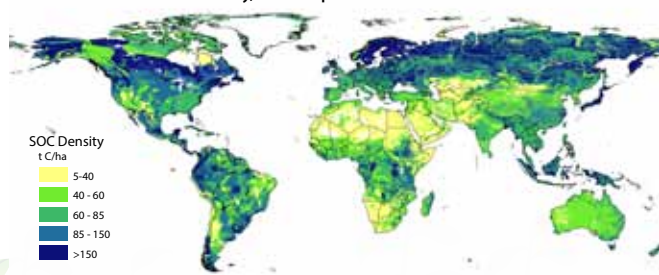
Global variation in SOC density, 0-1 m depth
