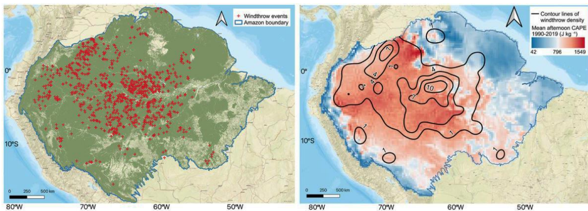
Figure 81: The spatial pattern of windthrows and mean afternoon convective available potential energy (CAPE). Left: 1012 Windthrow events identified manually using Landsat 8 images; green colour in the background represents forested area. Right: Contour lines of windthrow density (counts per 10,000 km 2 ) over the mean afternoon CAPE at 0.25° resolution [170]
