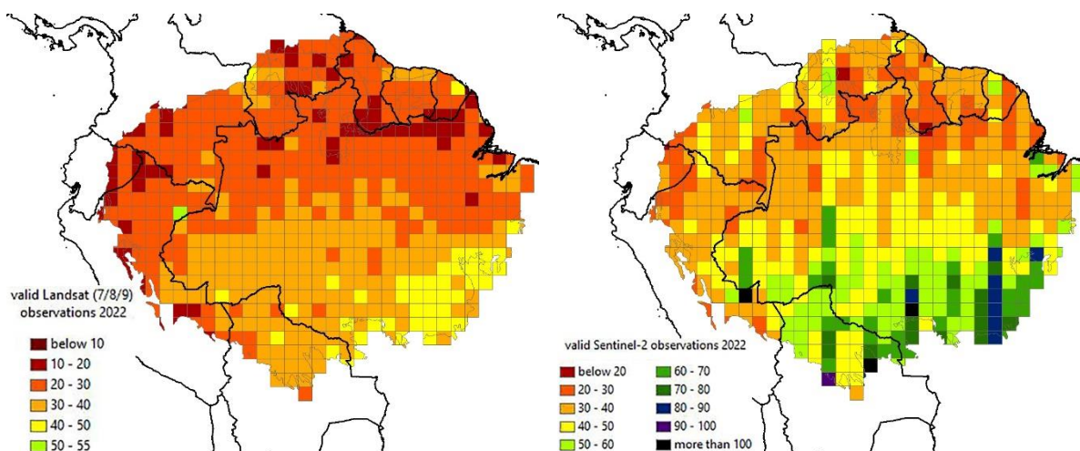
Figure 44: Average number of valid observations (VOs) per pixel for 250 km x 250 km grid cells in the Amazon region. Left: Landsat 7/8/9, right: Sentinel-2
