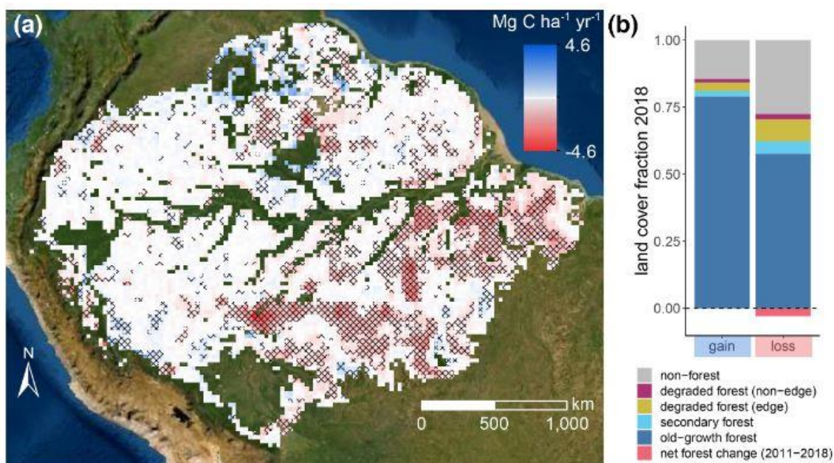
Figure 58: Trends in AGC and the associated forest cover fractions. (a) AGC trends (2011–2019) over the Amazon biome. Grid-cells where trends are significant are indicated with cross-hatches and cells where reliable data were not available are omitted (e.g. flooded areas and regional anomalies). (b) Mean land cover fractions in 2018 averaged over grid-cells showing significant positive (gain) and negative (loss) trends. Displayed are the proportions of old-growth, degraded (edge and non-edge), secondary forest and non-forest area. Edge degradation includes forest within 120 m distance from human-made forest edges. The net change in forest area fraction relative to 2011 is also indicated ( \sim 0 for gain cells, -0.03 or 4% reduction for loss cells) [148]
