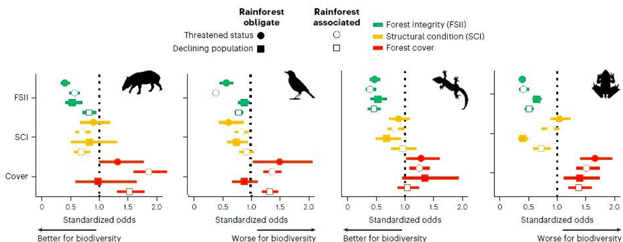
Figure 78: The relative importance of forest integrity, structural condition and forest cover on the odds of mammals, birds, reptiles and amphibians being threatened and having declining population trends. Forest integrity tended to be associated with a beneficial effect on biodiversity (lower odds of species being threatened and having declining population trends), relative to forest cover [167].
