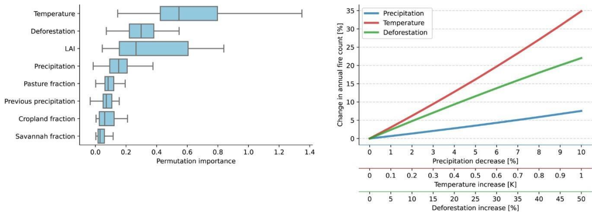
Figure 67: Permutation importance across all years (2003–2020) representing the importance of features for fire count prediction. Boxes show quartiles of the calculated permutation importance across individual years the median of which showing 50th percentile. Calculated permutation importance is taken as an average combination of neural network (NN) and XGBoost (XGB). Model (NN and XGB) prediction sensitivity showing annual change in total fires across the BAB as a function of incremental changes in surface temperature (+0.1 K to +1K), precipitation (–1% to –10%) and deforestation (+1% to +50%) calculated as an average across all years (2003–2020) [157].
