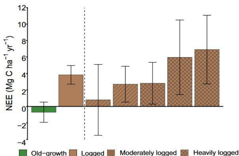
Figure 97: Net ecosystem CO 2 exchange (NEE) estimated by biometric ground-based methods. Left of the dashed line show the mean ( \pm 1 SE) of six unlogged forest plots (green) and five logged plots (brown) with error bars representing variation across the plots. Right of the dashed line show the logged plots individually: two moderately logged plots (striped) and three heavily logged plots (hatched) with error bars representing within-plot uncertainty, estimated by propagation of SEs of the individually measured components of productivity and respiration. Positive values indicate a net source of CO 2 to the atmosphere [187]
