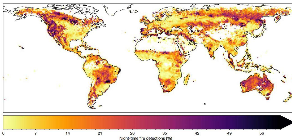
Figure 84: Large portions of the globe experience night-time fires. The map shows the percentage of 2003–2020 active fire detections ( n = 80,190,449 ) that occurred at night, from MODIS Fire Information for Resource Management System (FIRMS) data aggregated to 1^\circ resolution. The displayed pixel values are thresholded at 60% detection; less than 1% of the mapped land area had more than 60% of fire detections at night [176].
