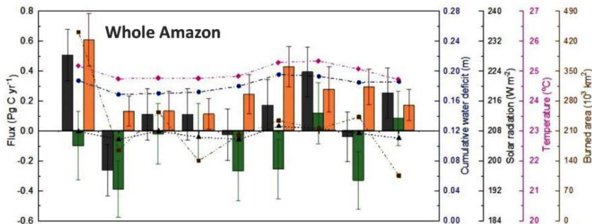
Figure 53: Annual mean carbon fluxes for the Amazon: : posterior total flux with the Amazon vertical profile observations in the inversion (black bars) and posterior fire fluxes using MOPITT carbon monoxide observations in the inversion (red bars). Annual cumulative water deficit (blue line), annual mean temperature (pink line), annual mean shortwave solar radiation downward flux (all sky; black line) and annual total burned area (brown line) [144]
