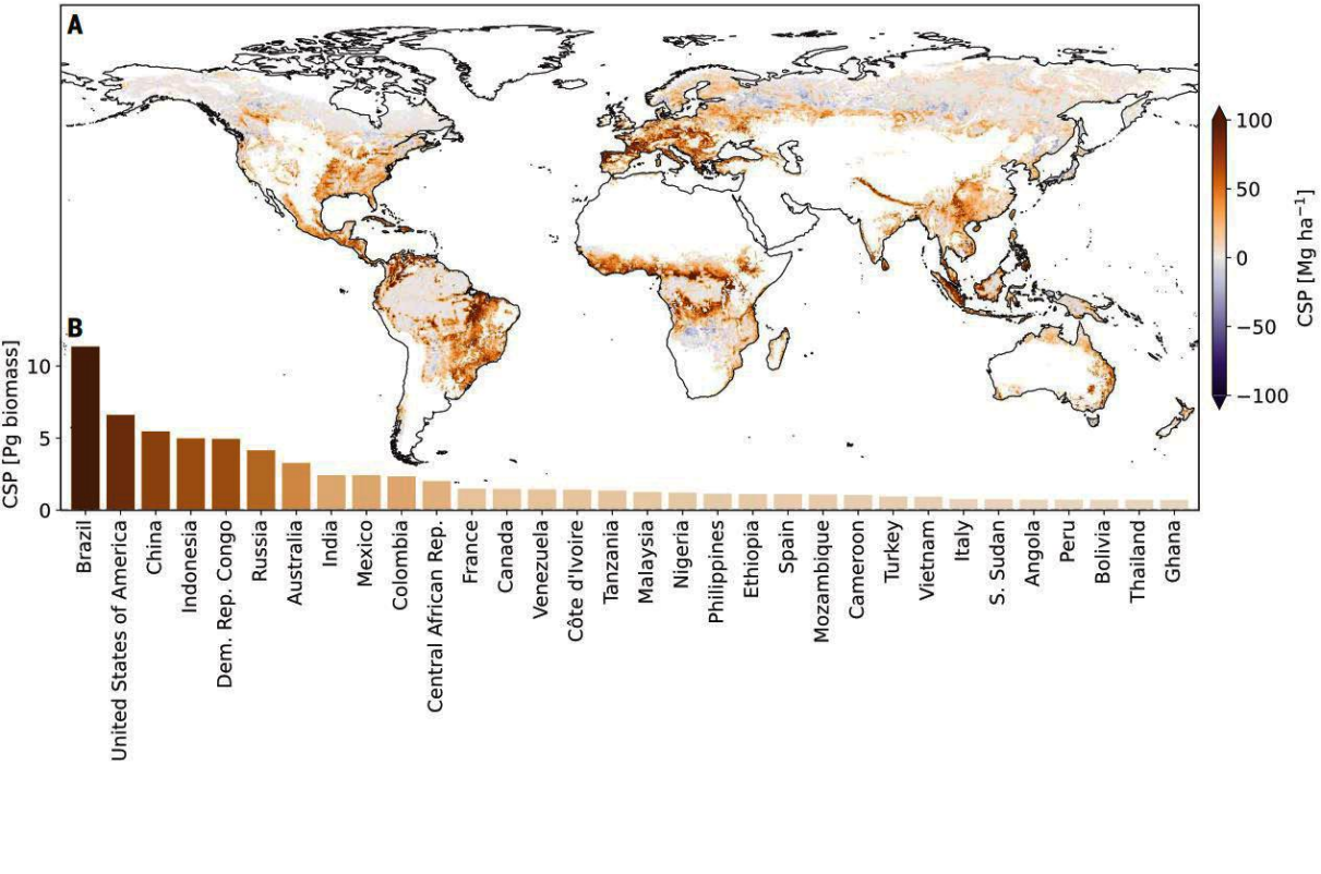
Figure 46: Additional carbon storage potential. (A) Additional carbon storage potential (CSP) in the hypothetical scenario in which all forests would resettle in their natural equilibrium if all direct human management was removed from them. The CSP is calculated from the difference between biomass carrying capacity and the expected biomass (the biomass that would occur under local conditions with the given natural disturbance regime and average intensity of human intervention). (B) National statistics of additional CSP for countries where absolute values exceed 0.7 Pg biomass [136].
