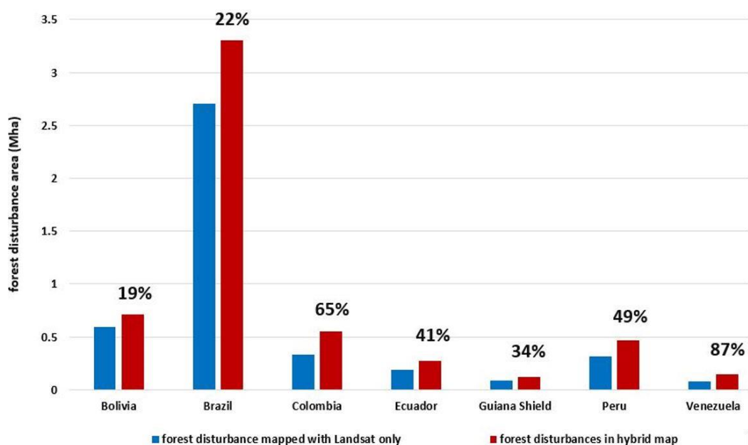
Figure 45: Moist forest disturbances 2022 mapped with a hybrid approach (Landsat, Sentinel-2), compared to the mapped forest disturbances with Landsat only. Surplus of the hybrid map is indicated as percentage
