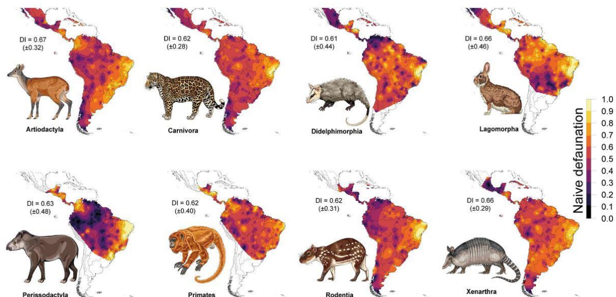
Figure 108: Interpolation-based geographic distribution of the naïve defaunation index (DI) broken down by mammal orders across the Neotropics. Maps were pruned by the averaged limit of the distribution of any mammal species within each order via a convex-hull approach [203].
