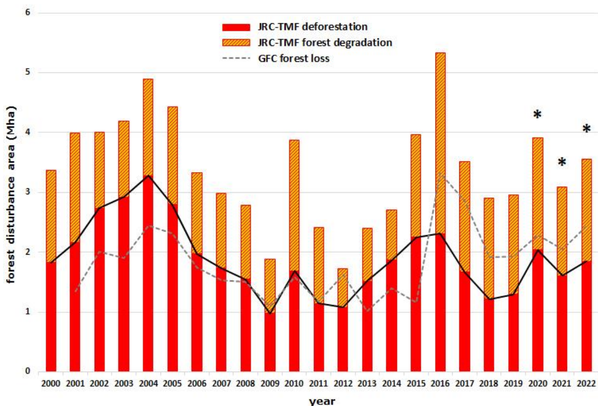
Figure 2. Forest disturbances in the Pan-Amazon humid forest from 2000-2022. The geographic basis are the areas of “Amazonia sensu stricto ” and “Guiana”, according to Eva and Huber [35]. GFC statistics appear as grey dashed line.
