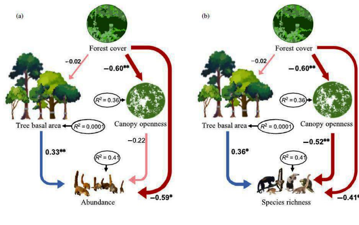
Figure 100: Path models of direct and indirect effects of forest cover on (a) abundance, and (b) species richness. Indirect effects of forest cover occur via two vegetation structural attributes (canopy openness and tree basal area). Significant pathways are indicated with asterisks (* p < 0.05 ; ** p < 0.01 ) to the right of the standardized path coefficients, while blue and red lines indicate positive and negative effects, respectively. Arrow thickness is scaled to illustrate the relative strength of the effects. The coefficient of determination ( R^2 ) is shown within black ellipses for all response variables [191].
