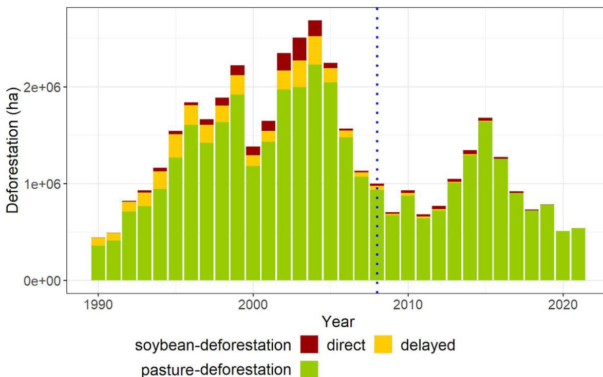
Figure 34. Deforestation in the Brazilian Amazon from 1990 to 2021 due to soy plantation within five years (red bars), soy plantation at least five years after the deforestation event (yellow bars), and permanent pasture (green bars). The dotted blue line marks the cut-off date of the Soy Moratorium. The chart is based on JRC-TMF and MapBiomas data.
