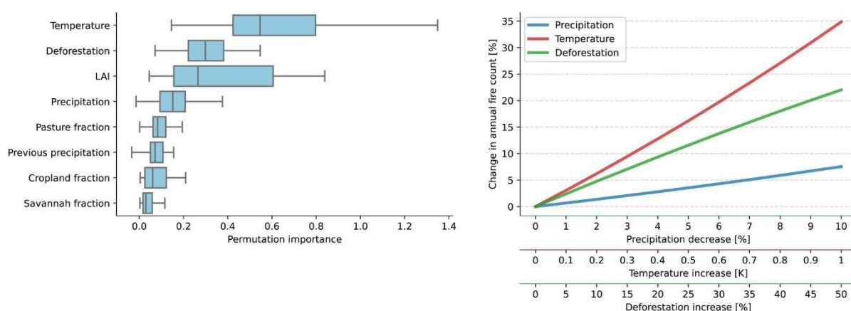
Figure 87: Left: Permutation importance across all years (2003–2020) representing the importance of features for fire count prediction. Boxes show quartiles of the calculated permutation importance across individual years the median of which showing 50th percentile. Calculated permutation importance is taken as an average combination of neural network (NN) and XGBoost (XGB). Right: Model (NN and XGB) prediction sensitivity showing annual change in total fires across the BAB as a function of incremental changes in surface temperature (+0.1 K to +1K), precipitation (–1% to –10%) and deforestation (+1% to +50%) calculated as an average across all years (2003–2020) [157].
