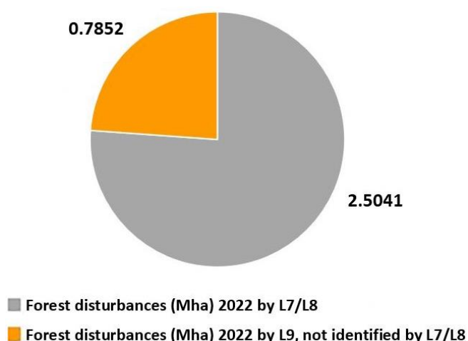
Figure 40: Comparison of mapped forest disturbance area 2022 (Pan-Amazon) with Landsat 9 and Landsat7/8 imagery
