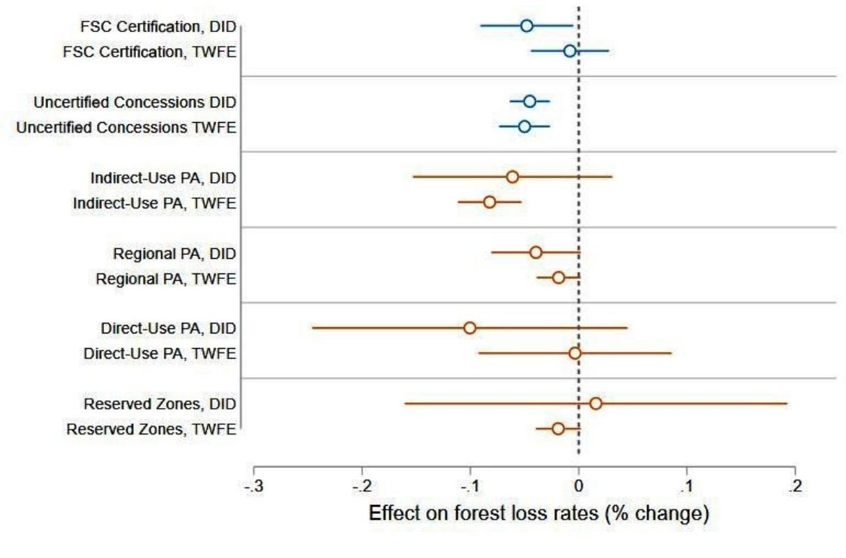
Figure 93: Comparison of forest loss impacts from different forest policies in the Peruvian Amazon, comparing the forest loss impacts of FSC certification and uncertified concessions estimated in this paper with the impacts of three different types of protected areas (PAs), as well as reserved zones in the Peruvian Amazon. Indirect-Use PAs are the strictest PA type. Direct Use and Regional PAs allow some resource extraction by local communities. Reserved Zones are transitory areas that are in the process of becoming a PA, so they are the least strict since they allow more economic activities [184].
