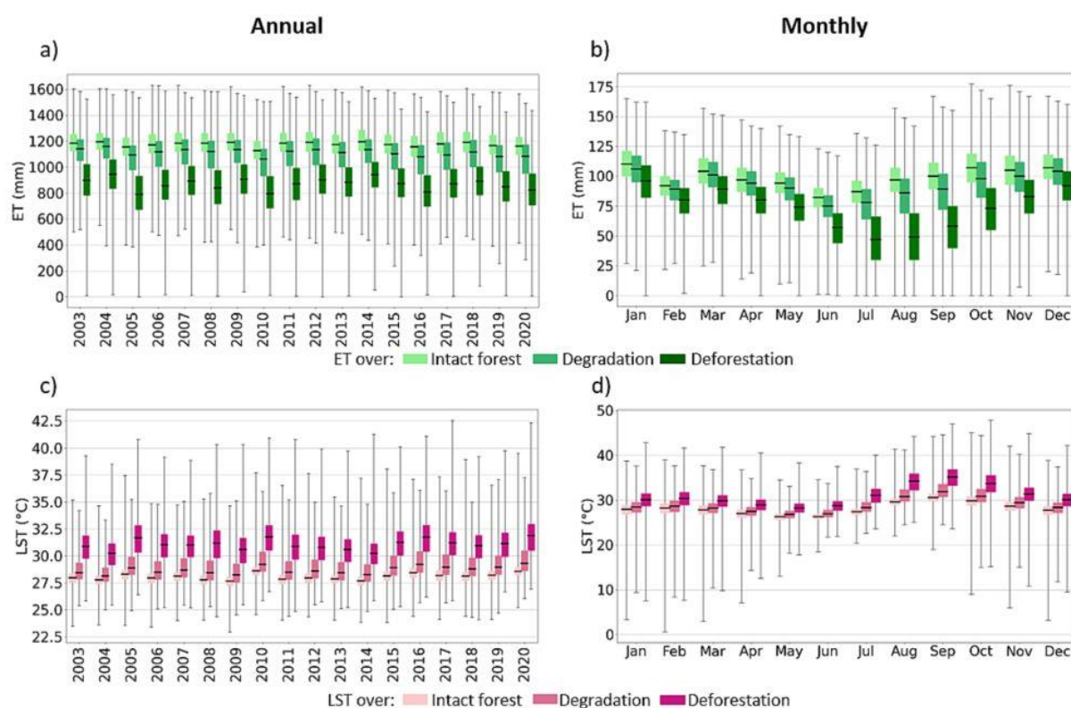
Figure 63: Data distribution of a) the annual ET totals, b) the average of the monthly ET totals, c) the annual LST averages, d) the average of the monthly LST averages over areas classified as intact forest, degradation, and deforestation in the entire study area [154].
