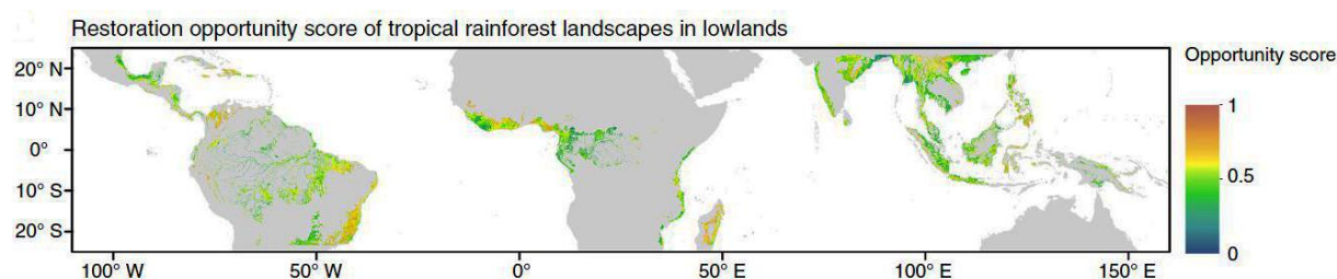
Figure 122: Restoration opportunity score in lowland moist tropical forest, indicating that restoration hotspots (i.e. clusters of red cells with a normalised score >0.8 ) exist across the tropics. Higher scores denote areas where appropriate restoration may maximise benefits (biodiversity conservation, climate change mitigation, climate adaptation, and water security) while increasing the likelihood of effective implementation and long-term sustainability (low land opportunity cost, lower deforestation rates in surrounding area, and higher likelihood of biodiversity recovery) [223]
