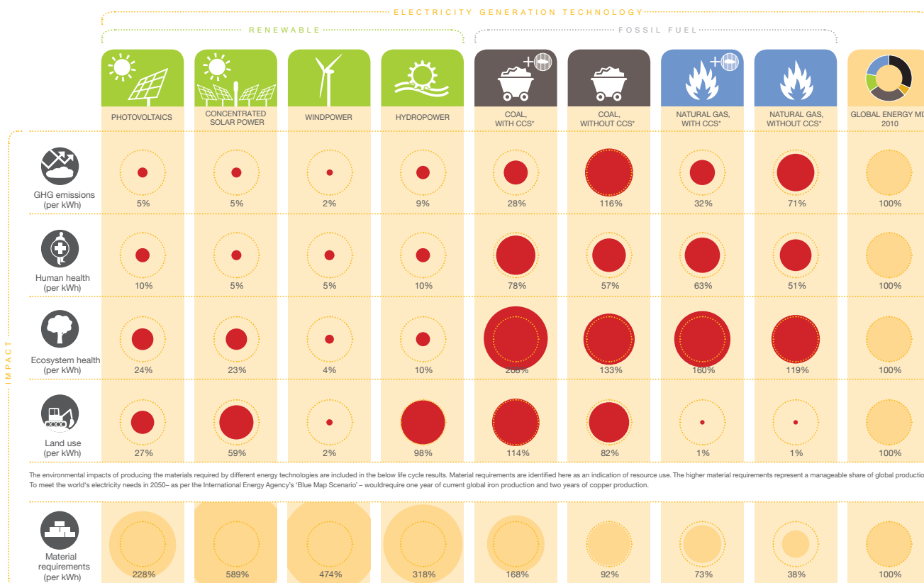
Figure 7: Overview over the life cycle impacts and material requirements of different technology groups compared to the global electricity generation mix in the year 2010
