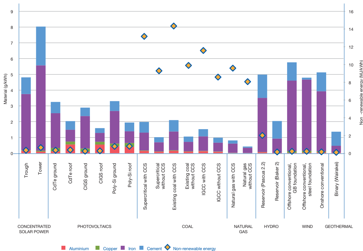
Figure 5: Bulk material and non-renewable energy requirements per unit power produced.
