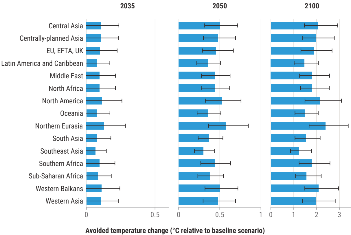
Figure 3.14: Changes in local temperature in the integrated action scenario, relative to the baseline scenario, 2035, 2050 and 2100, degrees Celsius.
