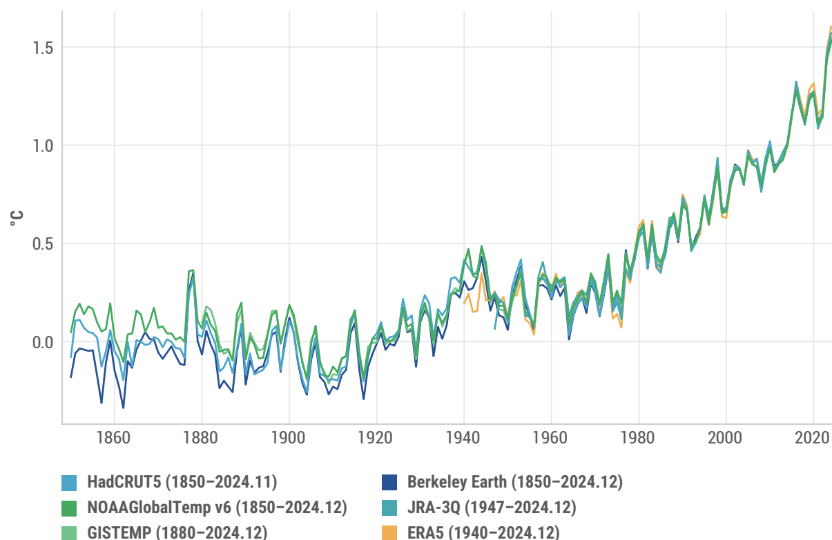
Figure 1.4: Observed global mean annual average temperature relative to the 1850–1900 average for the indicated datasets. Data Source: Copernicus Climate Change Service (C3S). Climate Indicators – Global surface air temperature.
