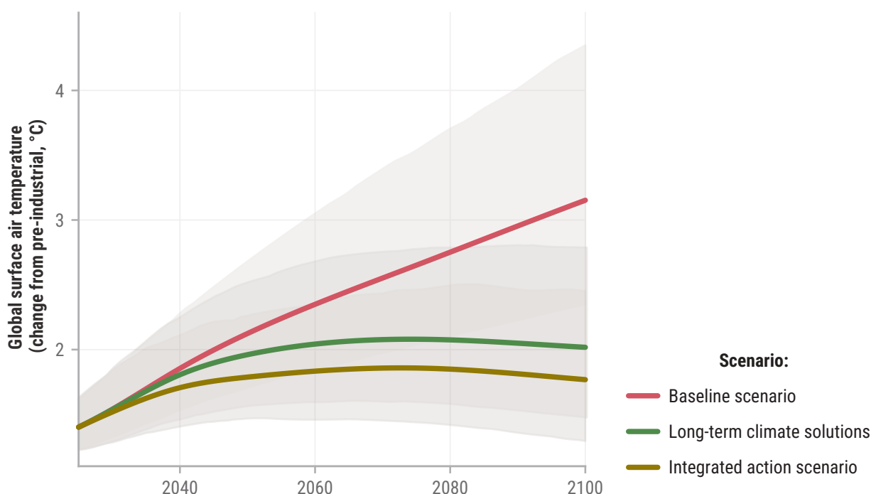
Figure ES2: Changes in global surface temperature for the baseline, the four long-term climate solutions and the full 25 integrated solutions (integrated action scenario) relative to pre-industrial levels, 2020–2100, degrees Celsius.
