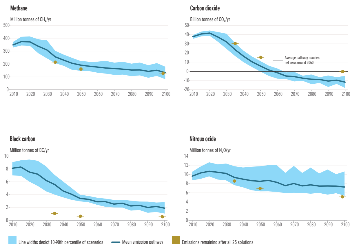
Figure 5.1: Net anthropogenic methane, carbon dioxide, black carbon and nitrous oxide emissions in the Intergovernmental Panel on Climate Change Sixth Assessment Report pathways limiting global warming to 1.5 °C with high overshoot (C2). The middle line shows the average emissions for all pathways, and shaded area shows 10–90 per cent ranges of these pathways. The gold dots show emissions reductions and residual emissions from implementation of the 25 measures in 2035, 2050 and 2100.
