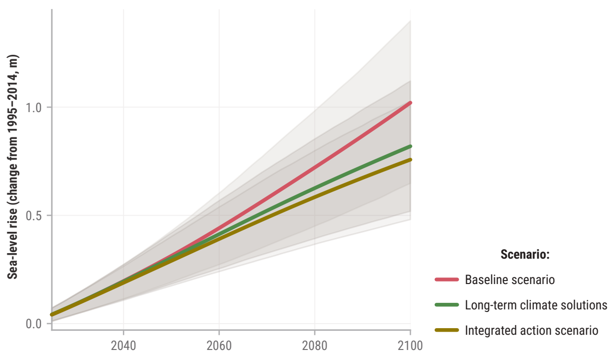
Figure 3.13b: Changes in sea level, for the baseline scenario, the four long-term climate solutions and the full 25 integrated solutions (integrated action scenario) relative to 1995–2014 averages, 2020–2100, metres.
