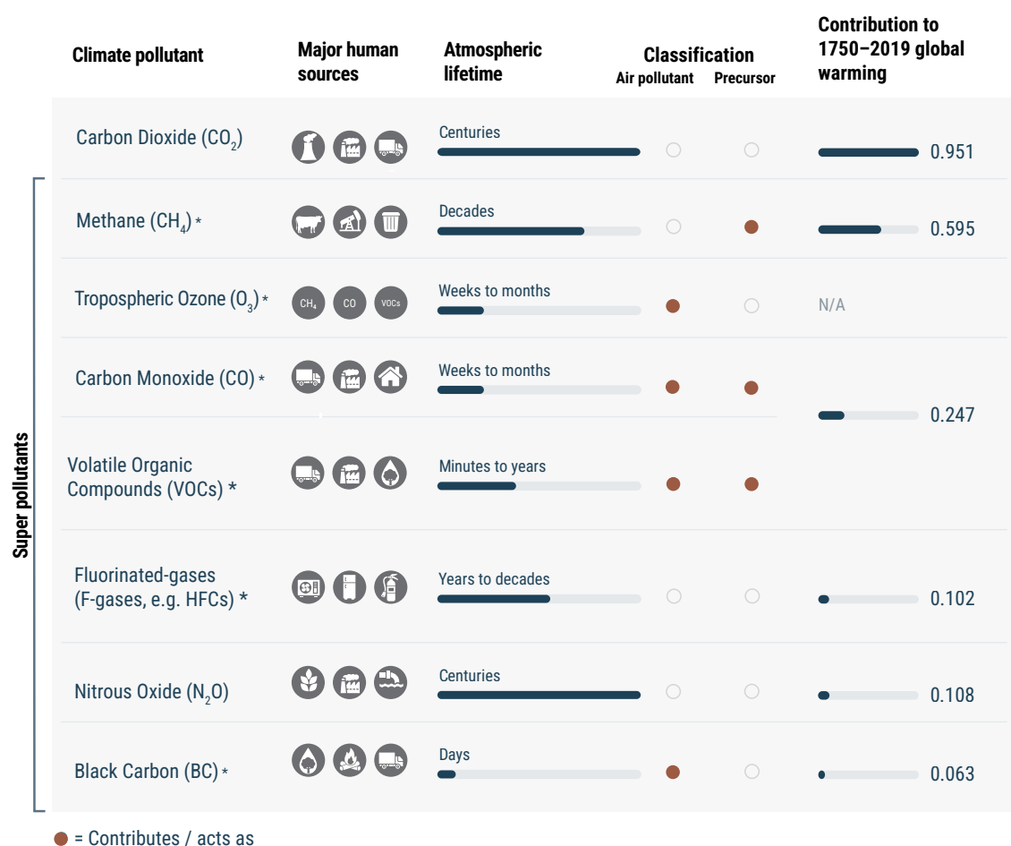
Figure 1.1: Climate pollutants, their major human sources, atmospheric lifetime, role as air pollutants or air pollutant precursors, and contribution to 1750–2019 global warming.
