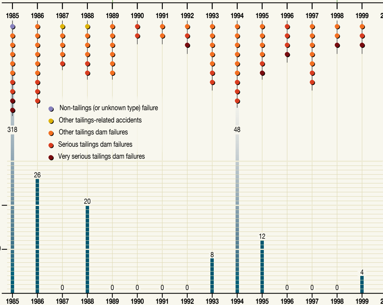
Figure 3. Timeline illustrating major initiatives to improve mine waste management and reported tailings dam failures (data from
